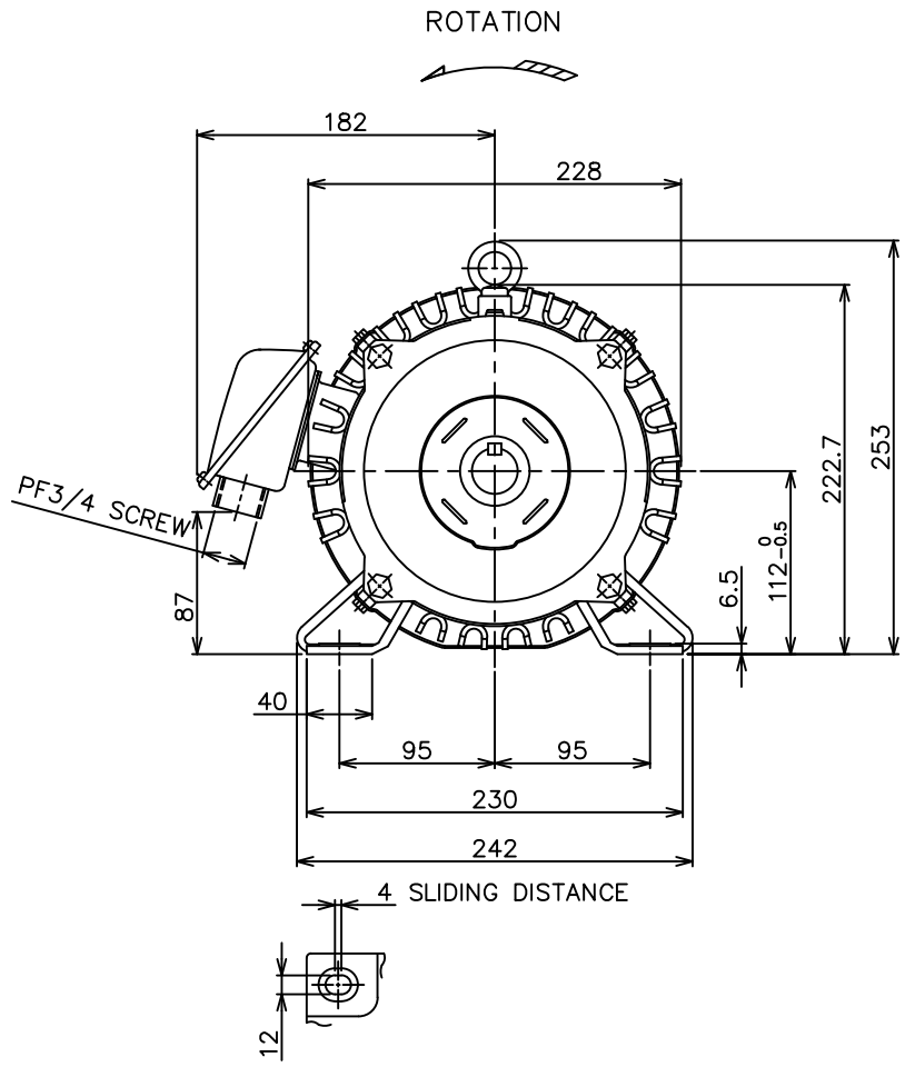
FRAME FOOT AS VIEWED FROM BELOW
